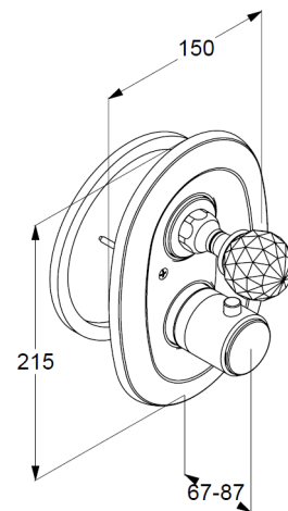
Dimensional drawing
